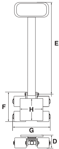
Trolley skates 4 wheels WLL = 4 t
