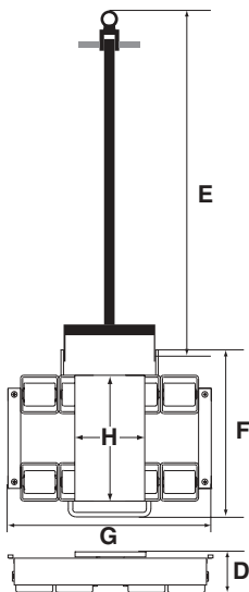
Trolley skates 8 wheels WLL = 6/8 t
